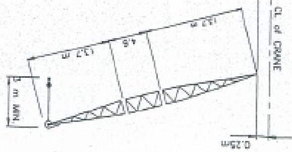
LOAD CHART M440D 30.0m RADIUS BOOM
